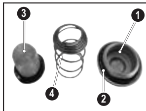
1. Palam Oil Strainer 3. Engine Oil Strainer 2. O-Ring 4. Spring
